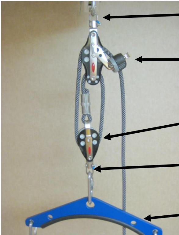
Height Adjustment System
